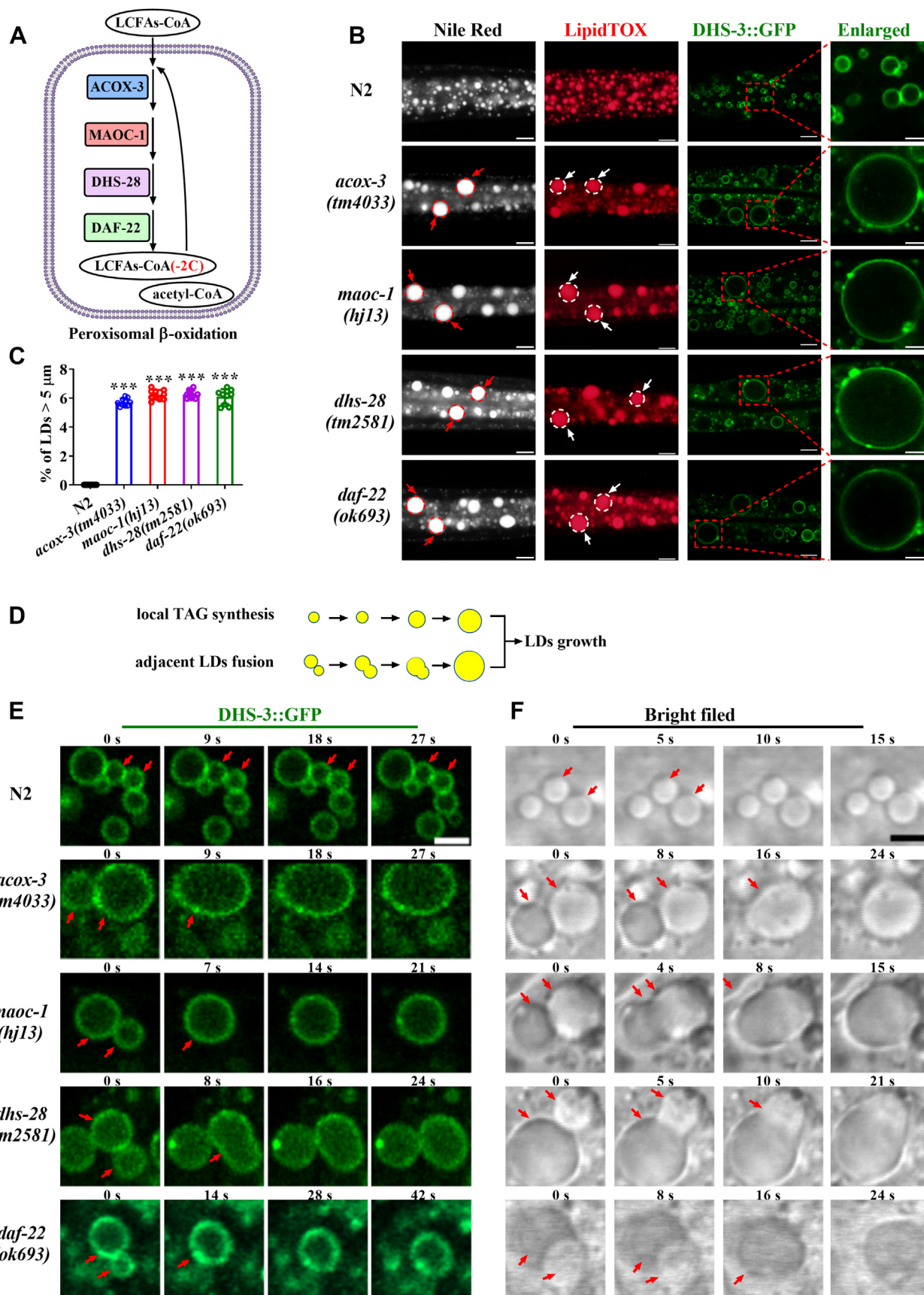
Figure 1. Dysfunction of peroxisomal \beta -oxidation pathway led to the formation of giant LDs (gLDs) in Caenorhabditis elegans . A , diagram of fatty acid catabolism by the ACOX-3/MAOC-1/DHS-28/DAF-22 peroxisomal \beta -oxidation pathway in C. elegans . B , lipid droplets (LDs) of L4 worms including the wildtype strain N2, acoX-3 ( tm4033 ), maoc-1 ( hj13 ), dhs-28 ( tm2581 ), and daf-22 ( ok693 ) mutants were visualized by postfixed Nile Red staining, postfixed
